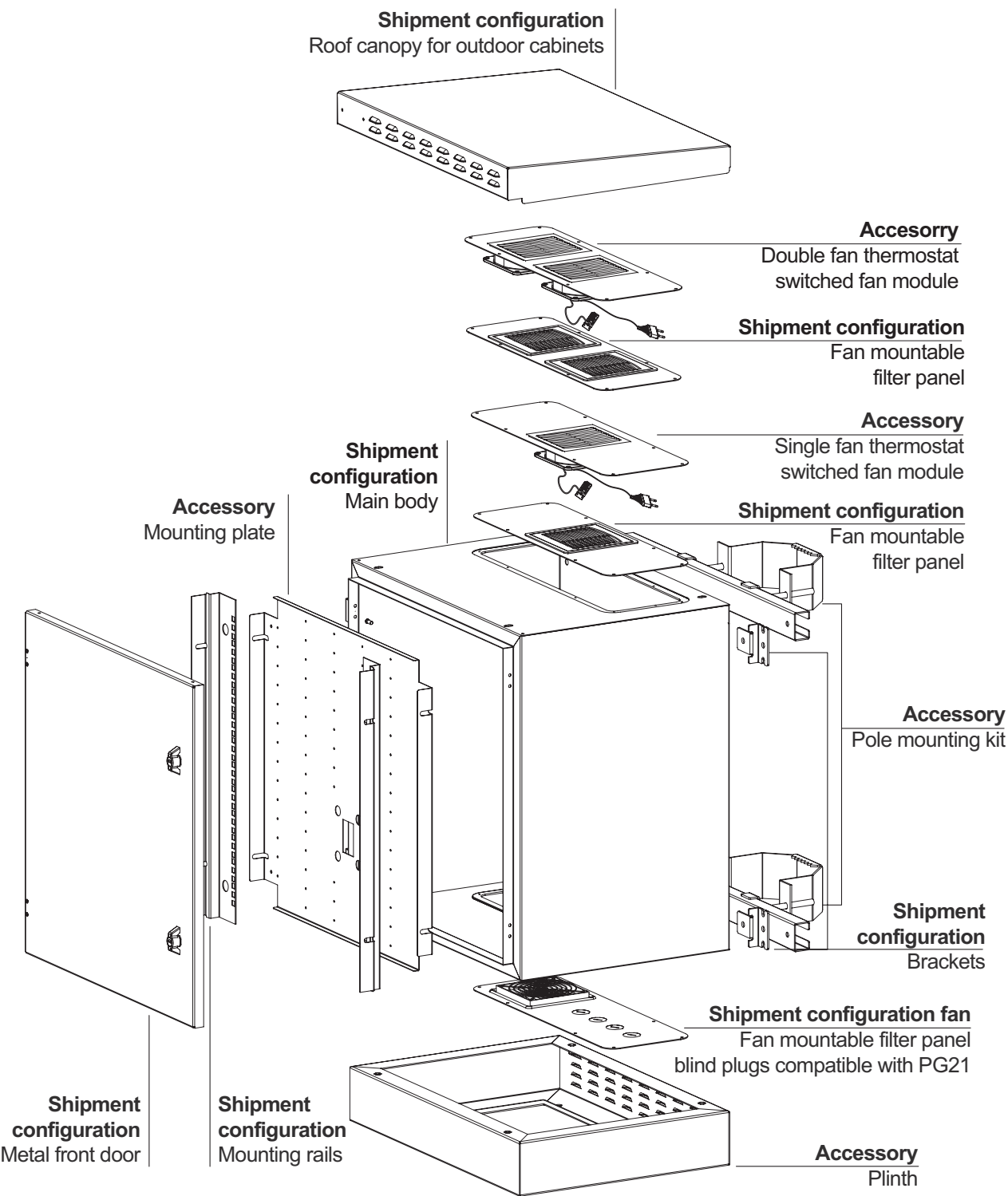
Exploded view
