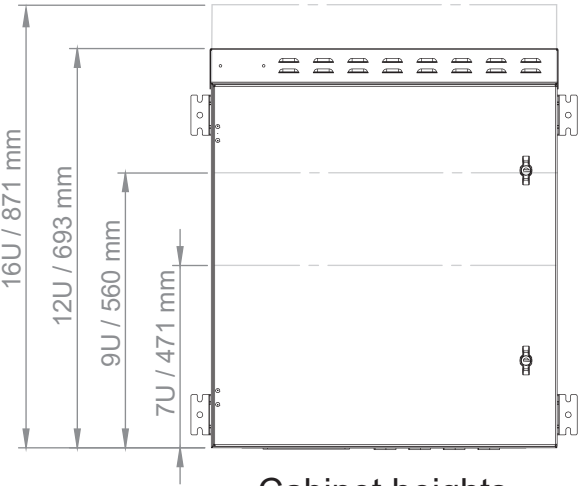
Cabinet heights
