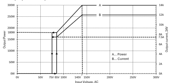
Output power - Output Current at 24V
